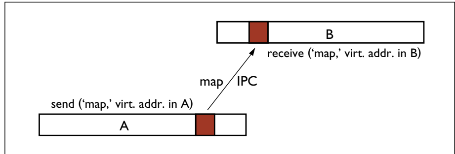
Figure 5. Recursively constructed address spaces
